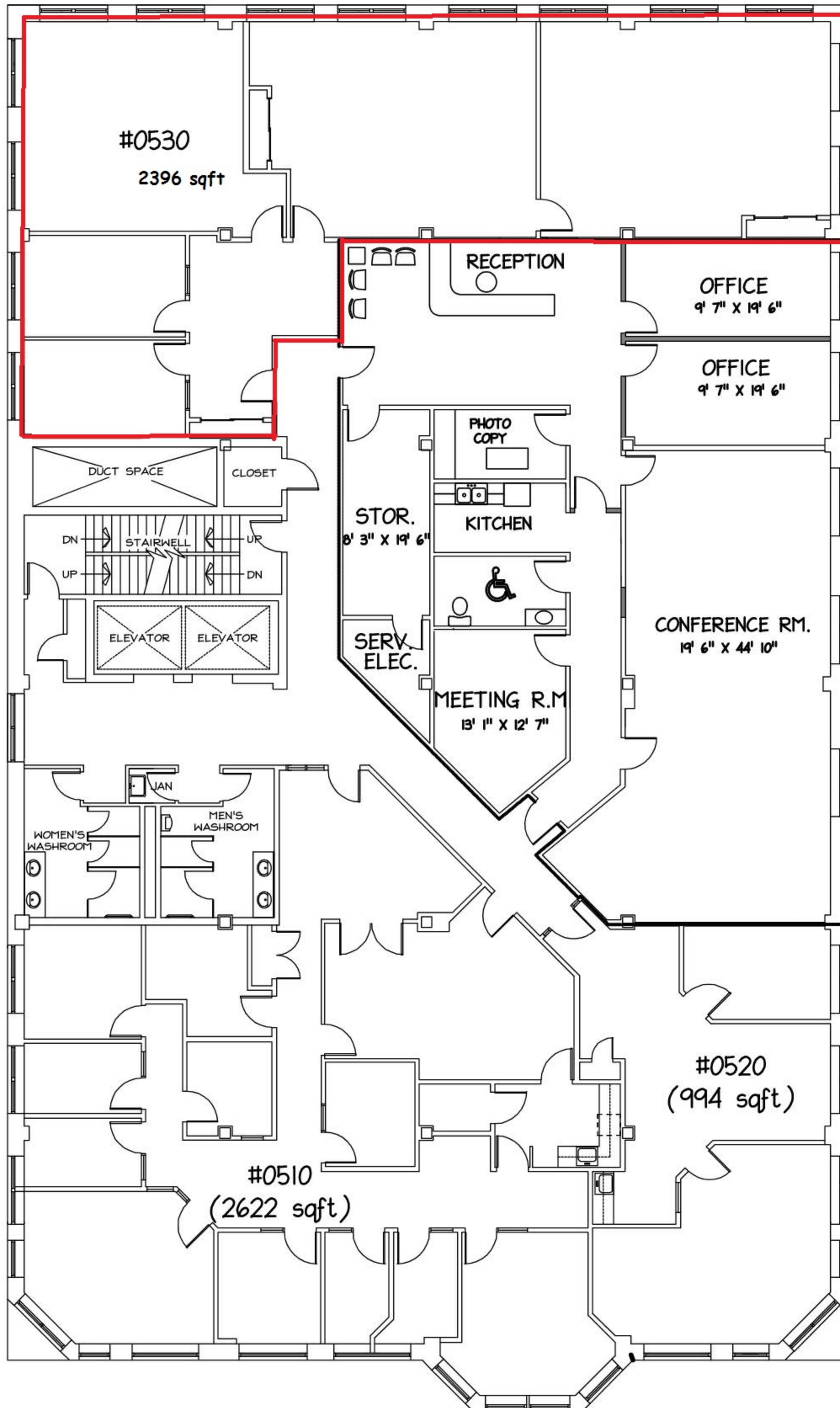
FIFTH FLOOR PLAN SCALE 1/16" = 1'-0"
